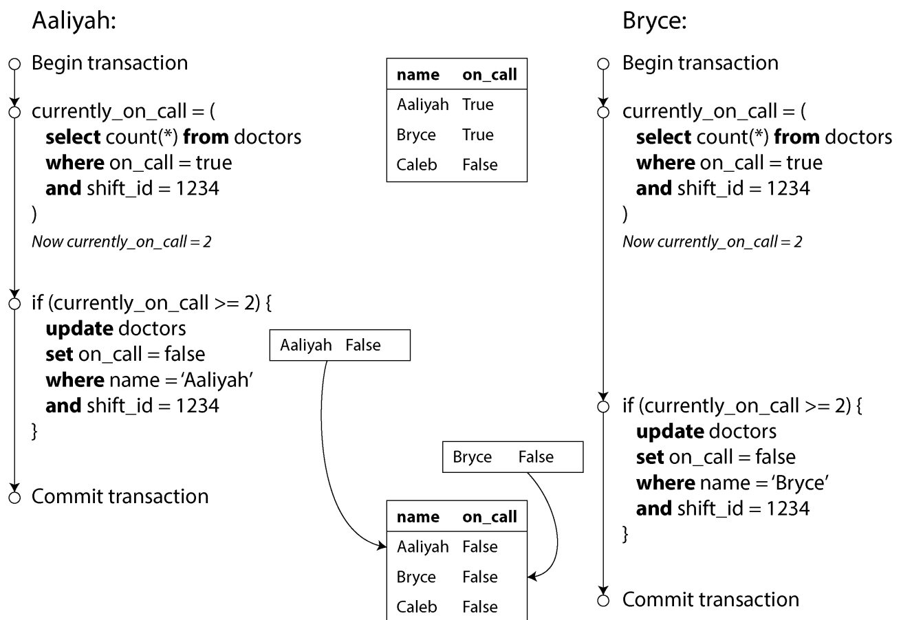
Figure 8-8. A write skew causing an application bug
