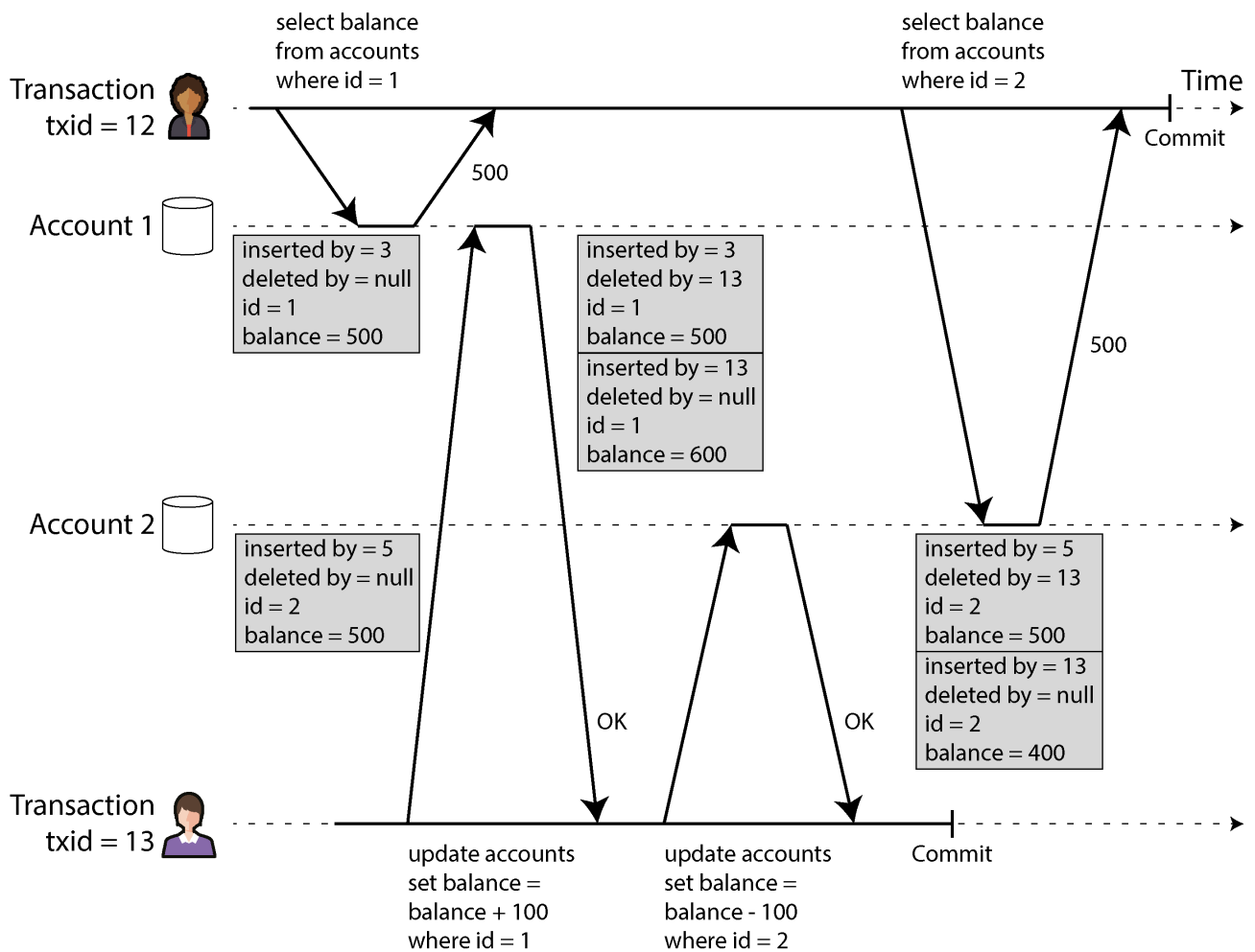
Figure 8-7. Implementing snapshot isolation using multiversion concurrency control
