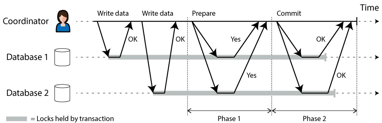
Figure 8-13. A successful execution of 2PC
